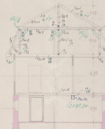
= Schnitt =
